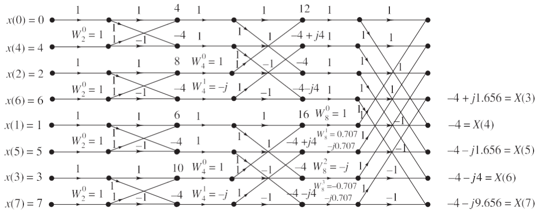
Figure 7.38 Computation of 8-point DF^{\dagger} of x(n) by radix-2, DI^{\dagger} FF^{\dagger} .
