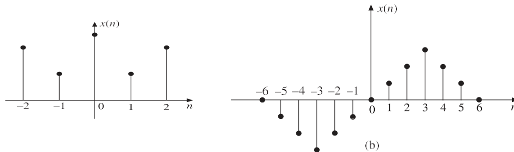
Figure 1.18 Discrete-time signals
