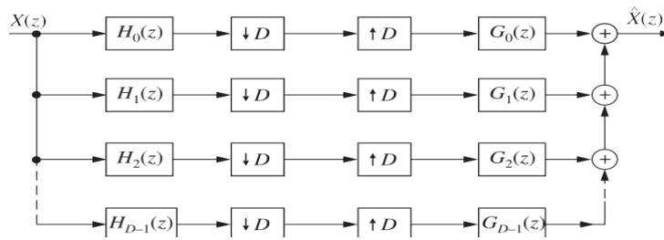
Figure 5.27 Sub-band coding filter bank.
